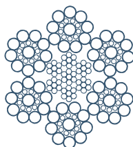
6 x 19 + AACI Seale 1-9-9
