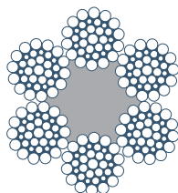
6 x36WS-AF WS 1-7-7+7-14
