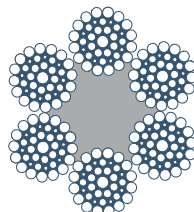
6 x41WS-AF WS 1-8-8+8-16
