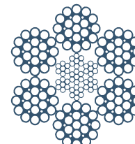
6 x 25 + AACI Filler 1-6-6F-12
